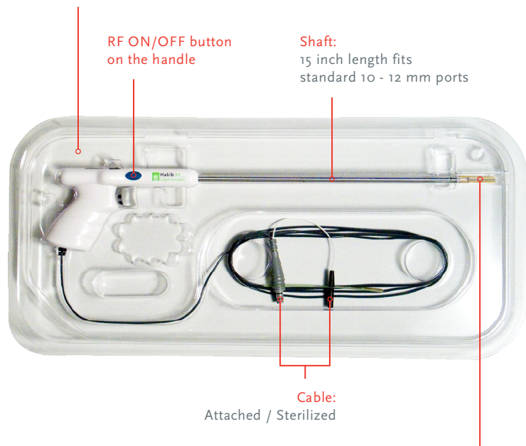
Electrode & Protective Plate: 3 cm length and char resistant with a push-off, depth-controlling mechanism
